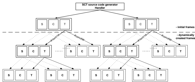
Fig. 1. The generation process
